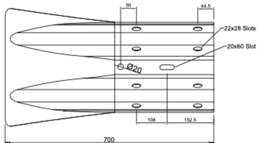
FACE VIEW
