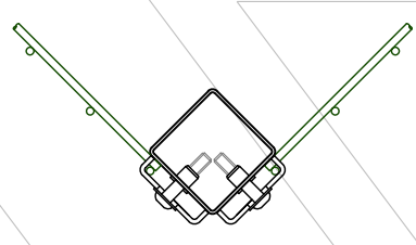
CORNER POST ARRANGEMENT
