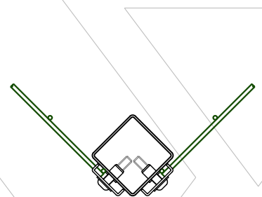
CORNER POST ARRANGEMENT
